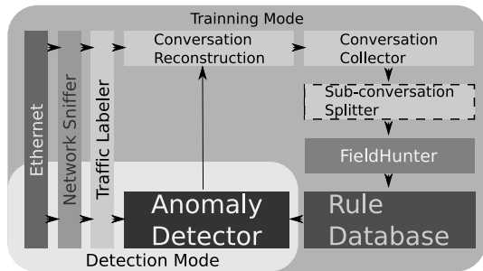
Figure 10: Payload Based Anomaly Detection System diagram.
