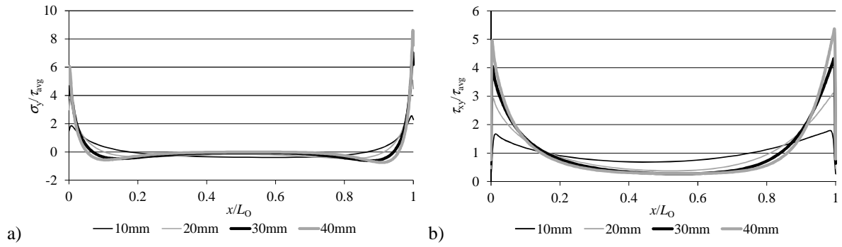
Fig. 6 – \sigma_y (a) and \tau_{xy} (b) stress distributions at the adhesive mid-thickness as a function of L_0 .
