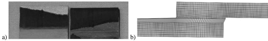
Fig. 10 – Representative experimental failure (a) and respective numerical prediction (b) for the joints with XNR6823 and L_O=10 mm.
