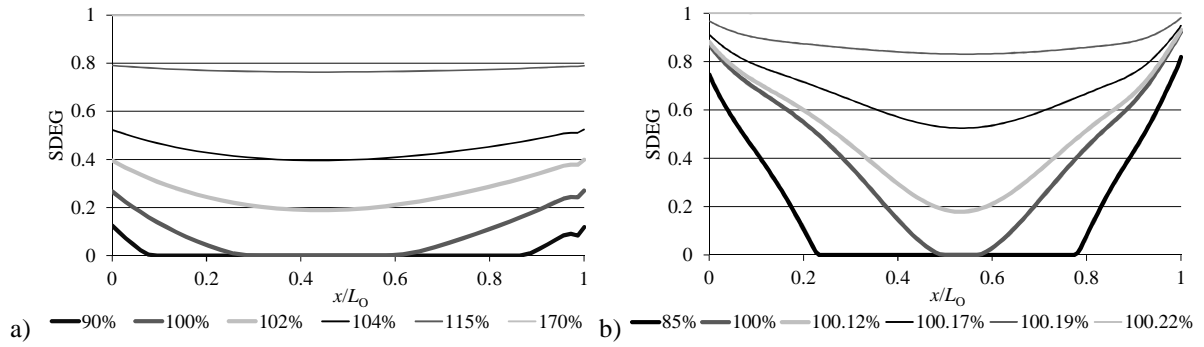
Fig. 9 – Evolution of the damage variable SDEG across the bondline (plane P4) with increasing values of \delta \delta_{Pmax} for the hybrid joints bonded with the XNR6852 and L_O=10 mm (a) and L_O=40 mm (b).
