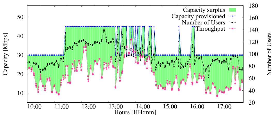
(b) Capacity provisioned and throughput (March 16, 2015).
