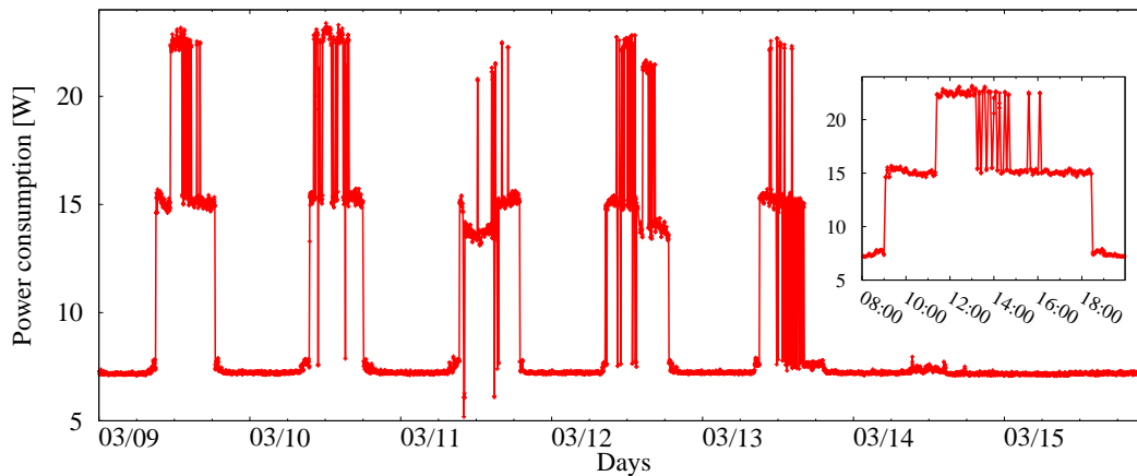
(a) Daily power consumption of a production network.
