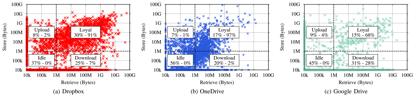
Fig. 3: Volume stored and retrieved by each household (in log axes). Households are divided in groups with limits at 1 MB. Labels report the percentage of households and bytes per group. Many idle households are seen in OneDrive and Google Drive.
