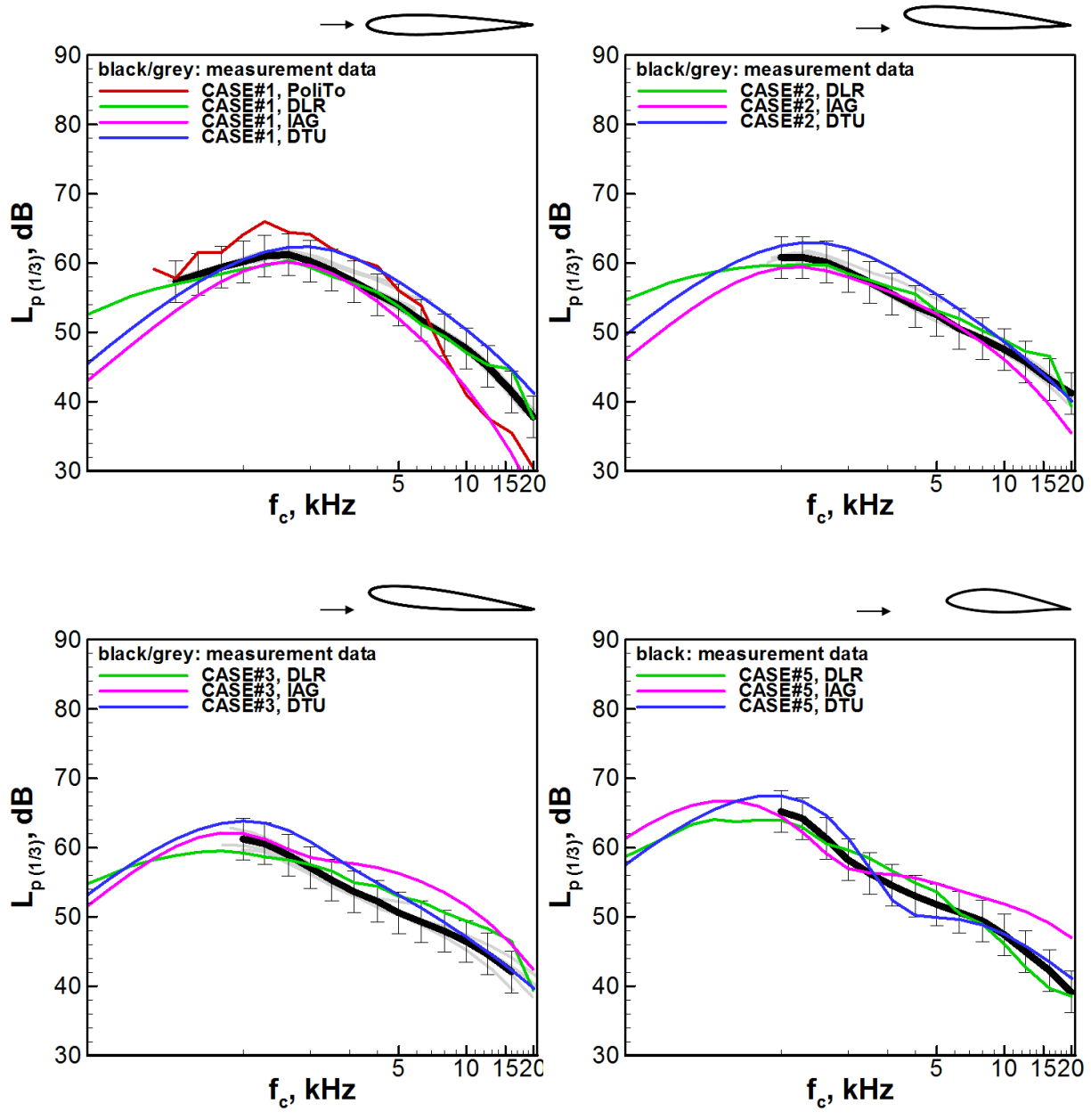
Figure 13. Overview of the achieved acoustic predictions compared to the measurement data. Experimental validation data from multiple facilities and research institutions, acquired with fundamentally different measurement techniques, are considered with a \pm 3 -dB scatter band.
