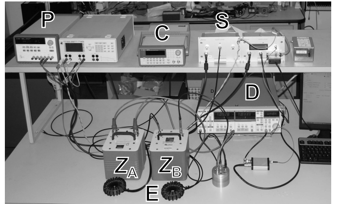
Fig. 4. Picture of the digital bridge showing the impedances Z_A and Z_B under comparison, the source S (energized by power supplies P , one for the analog and one for the digital part), the detector D and the coaxial equalizers E . A 10 MHz clock source C is also shown.
