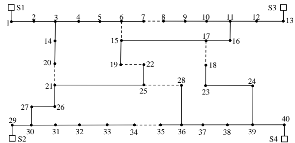
Figure 15. Globally optimal configuration with minimum losses for System E (dashed lines: open branches).
