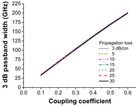
Fig. 4. 3 dB passband width as a function of coupling coefficients, with MRR diameter D = 20 \mu\text{m} .
