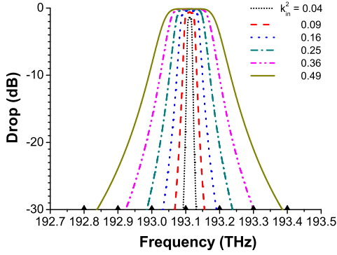
Fig. 3. Spectral response by varying k_{in}^2 , the coupling coefficients between bus waveguide and MRRs, with MRR diameter D = 20 \mu\text{m} and propagation loss 3 dB/cm.
