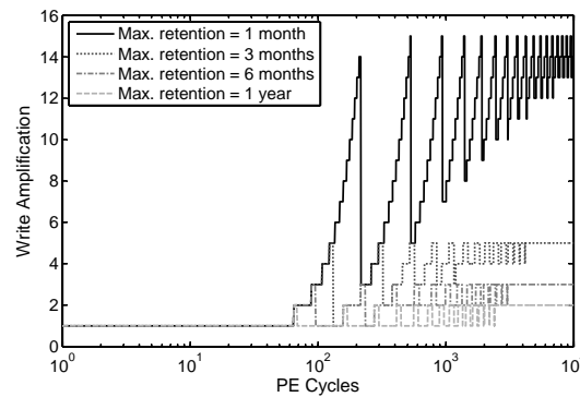
(a) FLARES Write Amplification for Videoserver application
