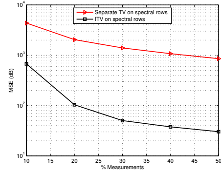
Fig. 5. Reconstruction of AIRS scene: 128 \times 128 x\lambda window.
