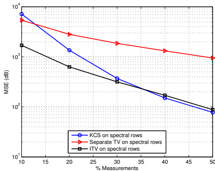
Fig. 4. Reconstruction of AIRS scene: 32 \times 32 x\lambda window.
