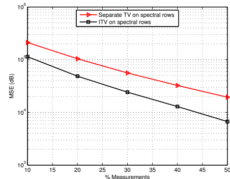
Fig. 6. Reconstruction of AVIRIS scene: 128 \times 128 x\lambda window.
