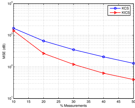
Fig. 3. Reconstruction of AIRS scene: 32 \times 32 xy window.
