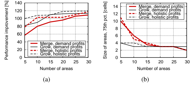
Fig. 2. Performance improvement (a) and area size (b) as functions of the number of areas, for different approaches and profit metrics.
