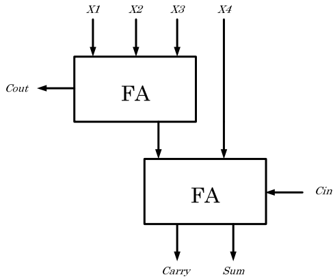
Figure 3. Implementation of 4-2 Compressor
