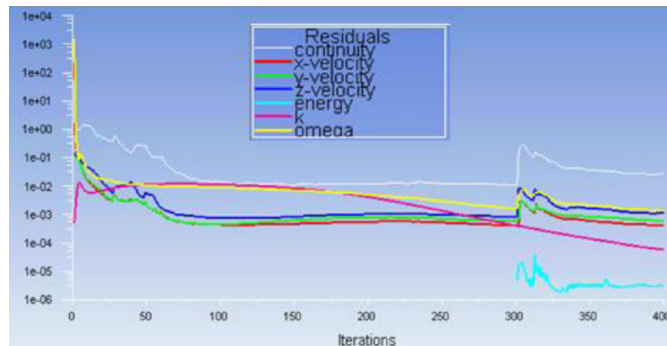
Fig. 31. Residual history in the thermal-hydraulic simulation of the Inb segment.
