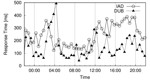
Figure 3. Evolution over time of average \Delta R for EC2 datacenters.
