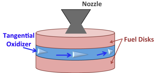
Figure 9: Vortex Flow Pancake engine scheme.
