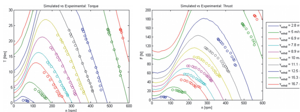
Figure 10 Experimental vs modeling results (aerodynamic-electric model)
