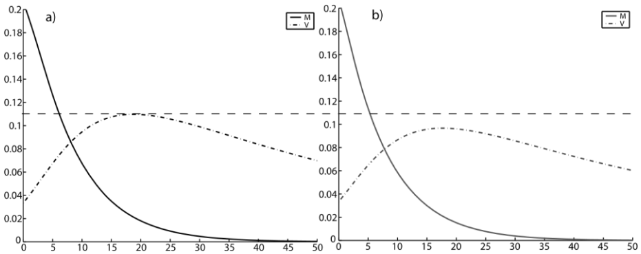
Fig. 4 Time-evolution of V and M for LU No. 24: (a) scenario A; (b) scenario B
