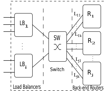
Fig. 1. MSSR Architecture: the load balancers (LB) (first stage), the switch (second stage) and the back-end routers (third stage)
