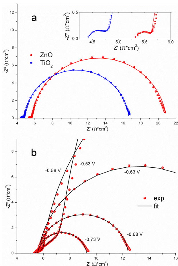
Fig. 7 (a) Measured (symbols) and fitted (solid line) EIS spectra at open circuit voltage of 18 μm thick ZnO-based and 8 μm thick TiO 2 -based DSCs. The high frequency zoom is reported in the inset. (b) High frequency behaviour of the ZnO based cell impedance: measurements (symbols) and fitting (solid lines) at applied voltage ranging from -0.53 V to -0.73 V with 0.05 V step.
