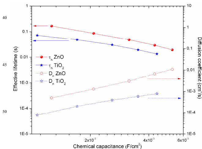
Fig. 8 Effective electron lifetime and diffusion coefficient dependence on the chemical capacitance for 18 μm thick ZnO-based and 8 μm thick TiO 2 -based DSCs.
