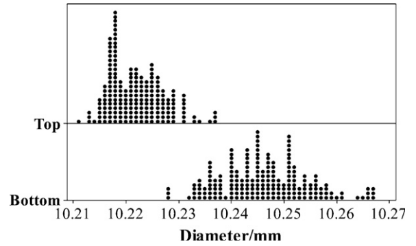
Fig. 6. Dotplots of measured values of diameter at bore's top and bottom.
