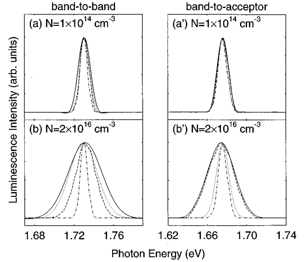
FIG. 7. Calculated spectral profiles of luminescence due to band-to-band- and band-to-acceptor recombination for carrier concentrations of (a), (a') 10^{14} \text{ cm}^{-3} and (b), (b') 2 \times 10^{16} \text{ cm}^{-3} . A carrier distribution generated by a 150-fs pulse is considered. The dash-dotted lines were calculated from a semiclassical model using a golden rule approach for the generation and recombination rate. For the dashed lines, the broadening of the generation process was taken into account while the recombination rate was calculated from the golden rule. The dotted lines were obtained with a golden rule generation rate and using a broadened recombination rate. The solid lines give the result when broadening of both generation and recombination processes are included. For band-to-acceptor luminescence, the broadening of the recombination process is negligible.
