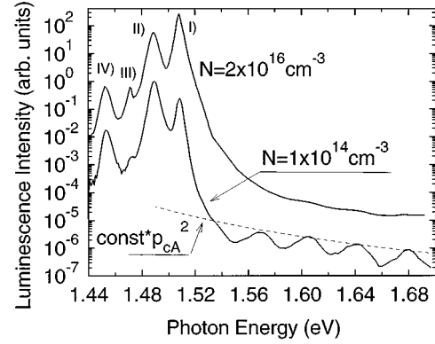
FIG. 1. Total emission spectrum of the p -GaAs sample measured with femtosecond excitation of N = 10^{14} and 2 \times 10^{16} electron-hole pairs per \text{cm}^3 . At low photon energies, we observe luminescence peaks due to recombination of thermalized electrons with free holes (I) and with bound holes (II). The peaks at lower energies originate from recombination processes of electrons with free holes (III) and bound holes (IV) involving simultaneous emission of a photon and an optical phonon. The emission at high photon energies is caused by band-to-acceptor recombination of nonequilibrium electrons (peak structure) and by a very weak background due to band-to-band recombination. The dashed line represents the square of the energy-dependent matrix element p_{CA} of the band-to-acceptor transition.
