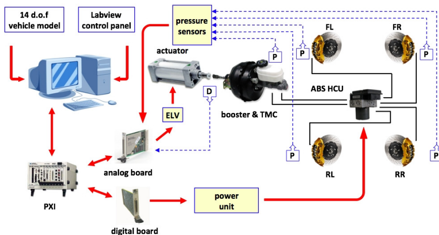
Figure 9: Layout of the experimental test bench, showing connections between brake plant and vehicle model (D: displacement and speed transducer, P: pressure transducers)
