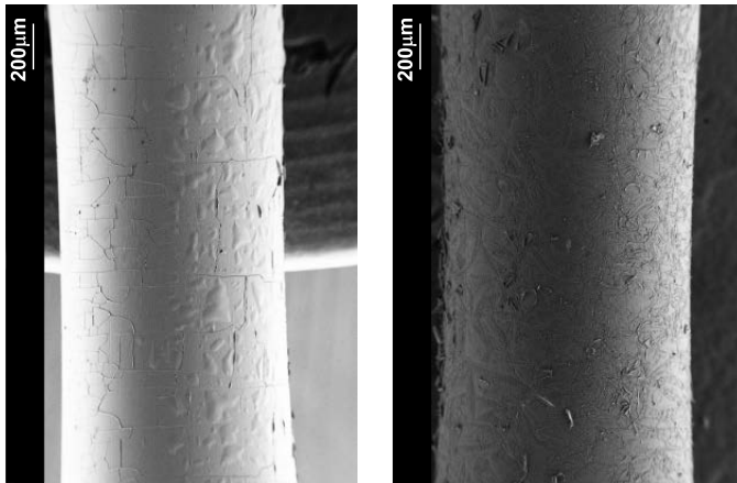
Fig. 8. FESEM images of coated fiber before (left) and after (right) the exposition to the HF vapors.
