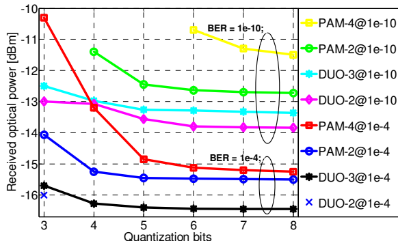
Fig. 4. Performance of the different modulation formats vs. the quantization bits in the receiver A/D converter in terms of required optical power for BER= 10^{-4} and 10^{-10} .
