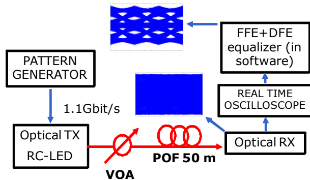
Fig. 1. Experimental setup plus eyediagrams before and after equalization.
