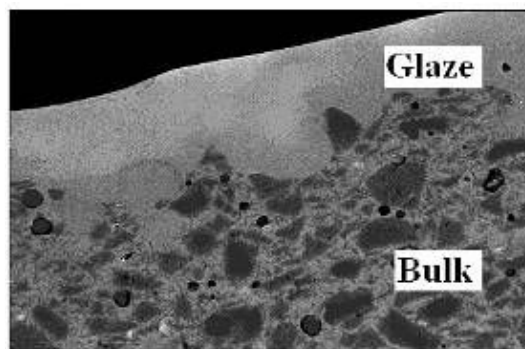
Fig.6: In the cementation method, the object is formed and dried. Then, it is buried in a glazing mixture (the cement) consisting of alkalis, copper compounds, calcium oxide or hydroxide, and/or quartz [13]. Upon firing, at about 1000 °C, a glaze layer is formed on the faience surface, and, around the object, a capsule. After firing, the cementation mixture can be crumbled away from the object, which is now coated with glaze.
