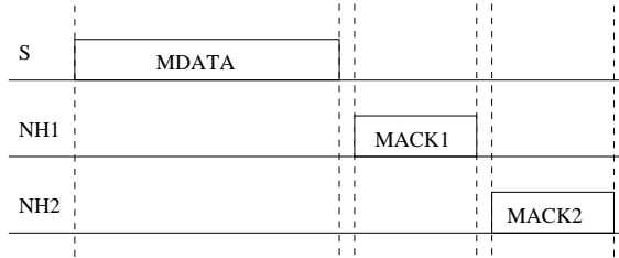
Figure 5: Transmission procedure used in RM^3 for multicast packets (except for the first one)
