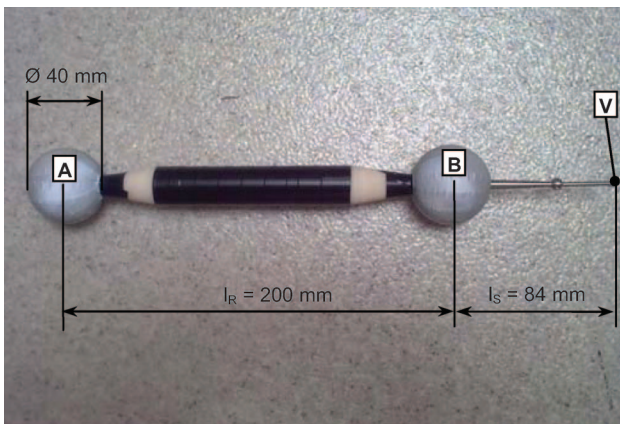
Figure 5. Mobile hand-held measuring probe.
