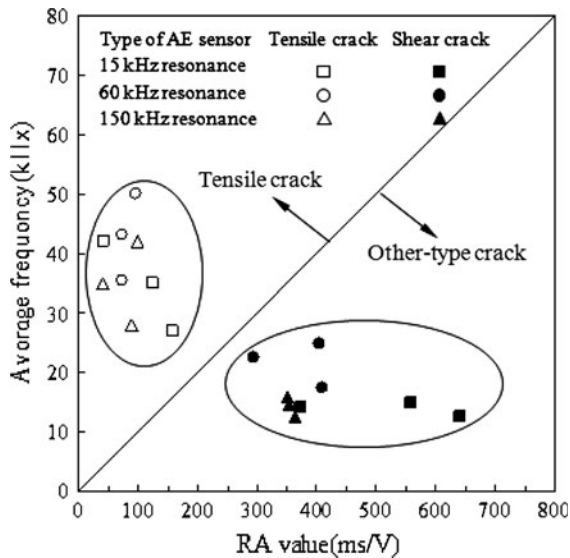
Fig. 2 Qualification of the damage by AE parameters
