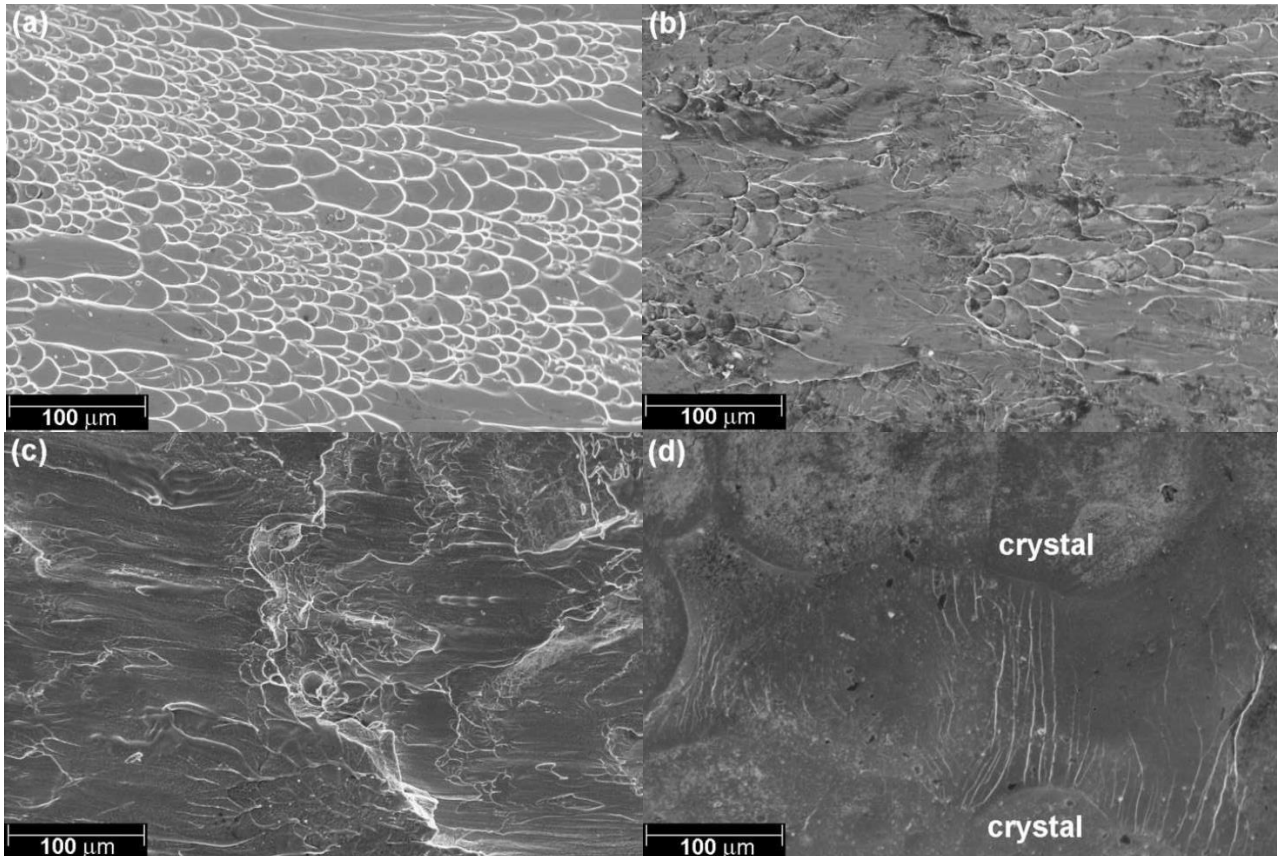
Fig. 4. Representative SEM fracture surfaces of the following samples: (a) fully amorphous Al 5 -3_(i); (b), partially crystalline (~ 23%) Al 4 -2_(i); (c) highly crystalline Al 4 -2_(iii). (d): external surface of Al 4 -2_(iii'), highly crystalline, undergone to compressive deformation.
