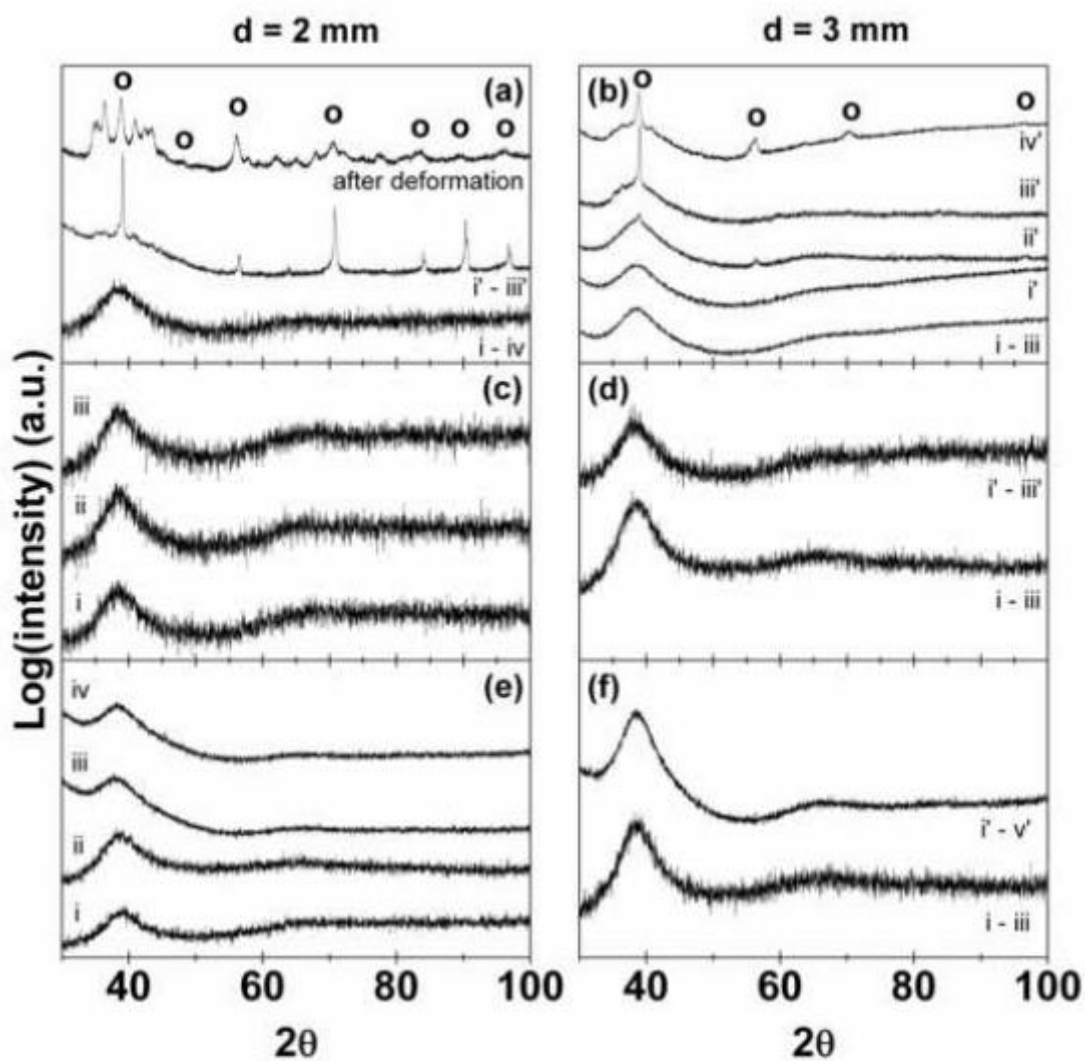
Fig. 1. Selected XRD patterns of different rods from the as cast rods. (a) and (b): \text{Cu}_{48}\text{Zr}_{48}\text{Al}_4 with 2 and 3 mm diameter, respectively; (c) and (d): \text{Cu}_{47.5}\text{Zr}_{47.5}\text{Al}_5 with 2 and 3 mm diameter, respectively; (e) and (f): \text{Cu}_{46.5}\text{Zr}_{46.5}\text{Al}_7 with 2 and 3 mm diameter, respectively.
