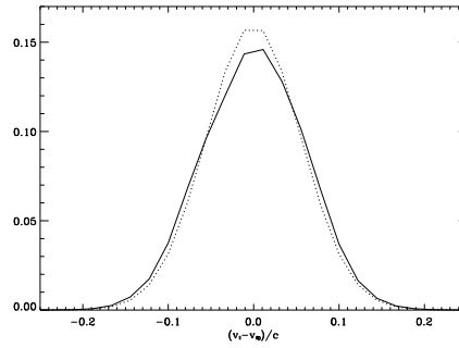
Figure 9. Profile of the distribution function of electrons as function of their parallel velocity normalized to the speed of light (continuous line). The dashed line represents the distribution function at t = 0 m. The figure refers to the case \rho_i = 0.004 m. As in fig. 8, the distribution function has been normalized to the total number of particles.
