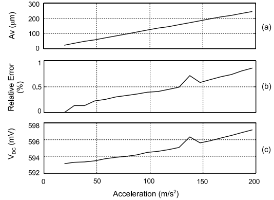
Fig. 6. Experimental results obtained at constant frequency ( 143 \text{ Hz} ) for different accelerations: (a) measured vibration amplitude (b) relative difference between the optical sensor and the accelerometer outputs (c) average value of the detected optical signal v_{DC} .
