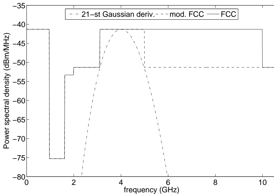
Figure 1: FCC masks, original and modified, and 21-st Gaussian power spectral densities.
