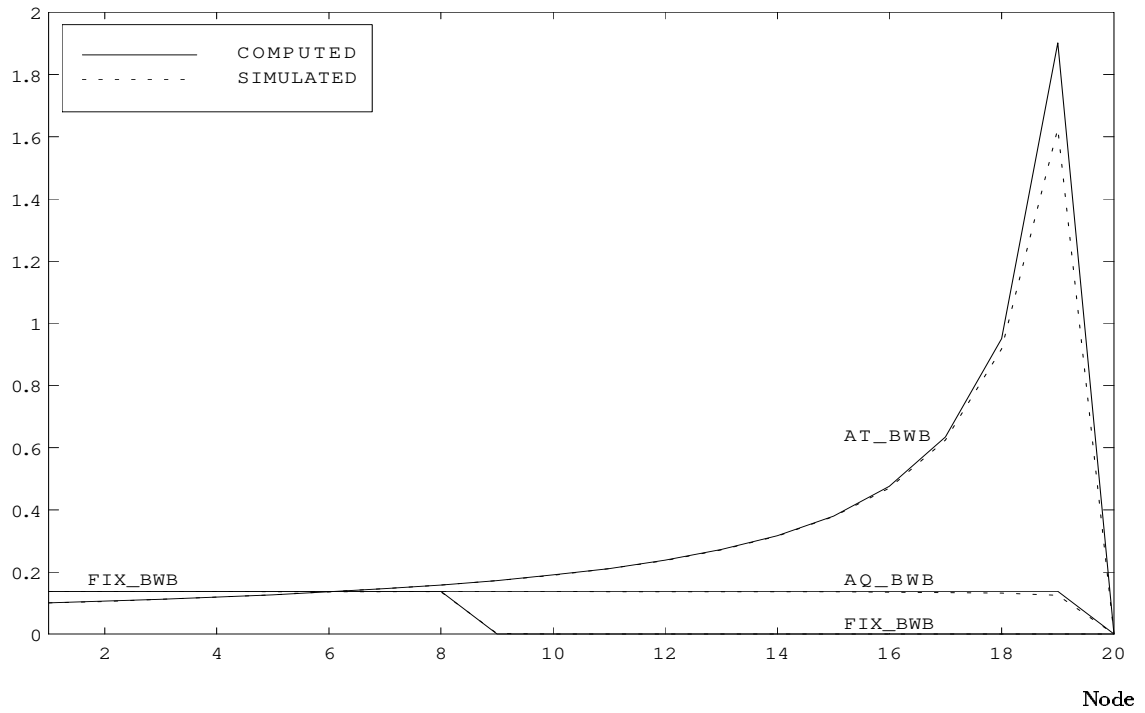
Figure 11: Delay time on bus A in steady-state overload condition.
