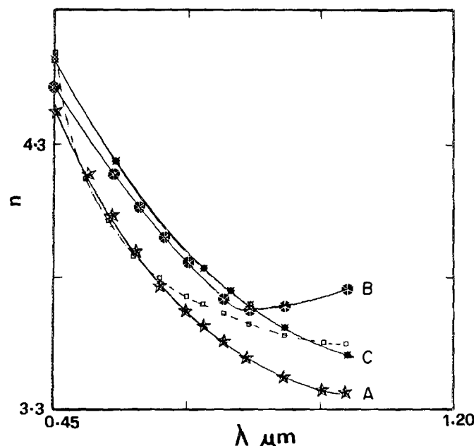
FIG. 6. n vs \lambda for a -Si:H films prepared by glow discharge compared with crystalline silicon (data taken from Ref. 52). Symbols: \triangle A ( T_s = 195^\circ\text{C} ); \bullet B ( T_s = 325^\circ\text{C} ); \blacksquare C ( T_s = 420^\circ\text{C} ).
