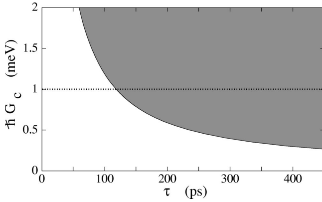
FIG. 2. Plot of the parameter space available (shaded area) for Eq. (3) in the implementation of \int_0^T \tilde{V}(t) dt = 2\pi .
