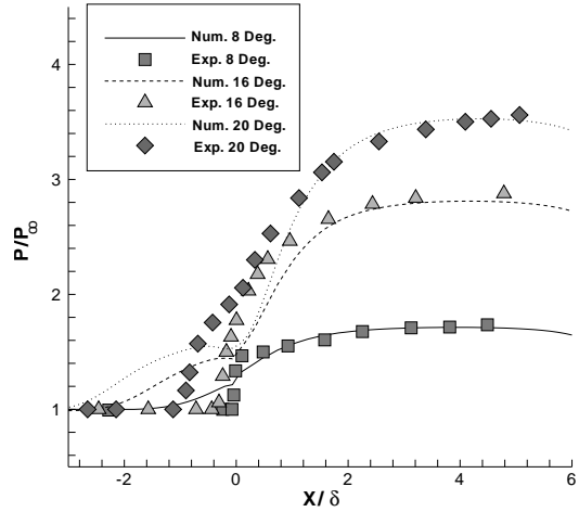
Figure 14: Supersonic ramp. Pressure comparison between numerical and experimental data
