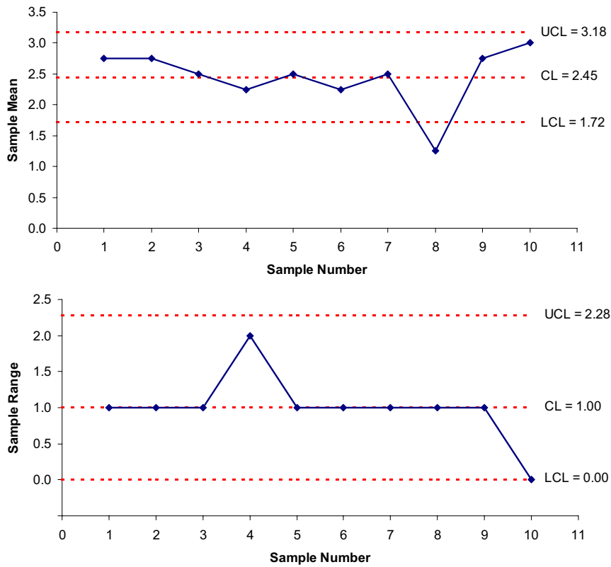
Figure 1. \bar{X} - R control charts for the example of visual control of the quality of a surface finishing of a mechanical part. The levels of the ordinal evaluation scale are numerically coded ('Low' = 1; 'Medium' = 2; 'High' = 3)
