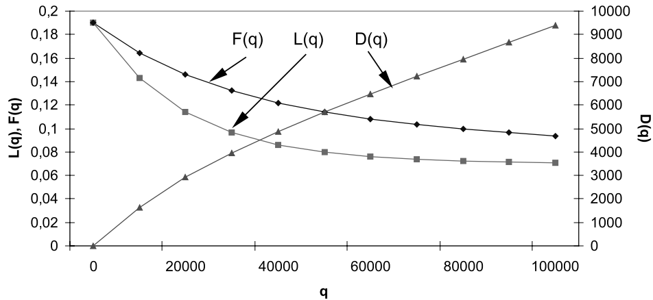
Figure 4. Comparison between D(q) , F(q) and L(q) for a generic manufacturing process.
